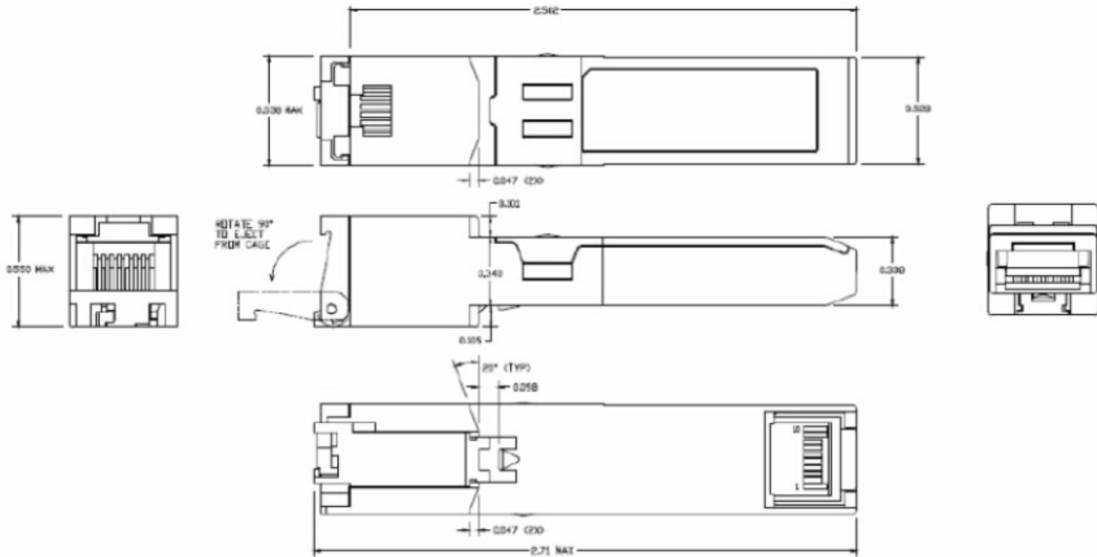
Figure2. Mechanical Specifications
