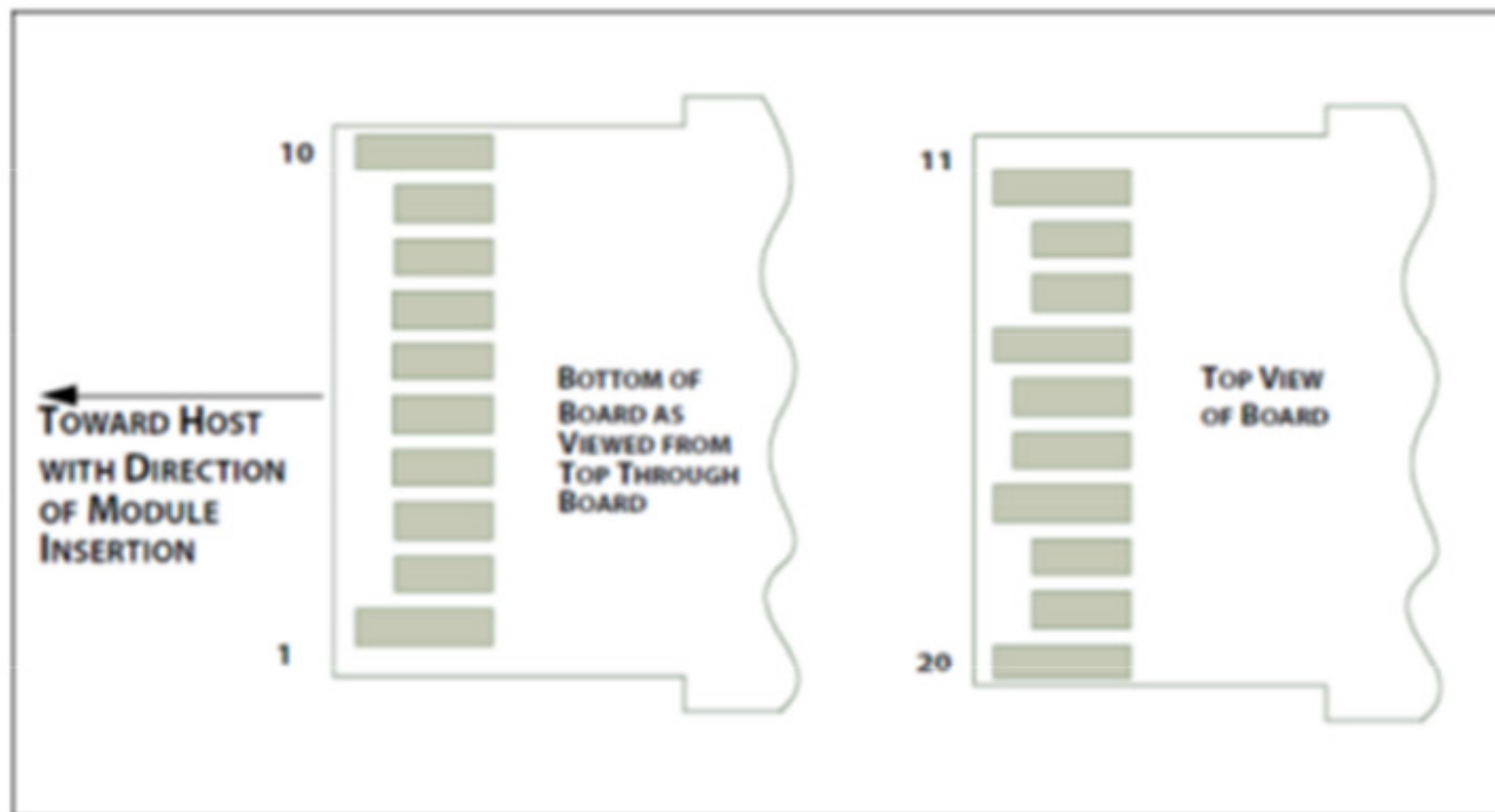
Figure 2: Module Contact Assignment
